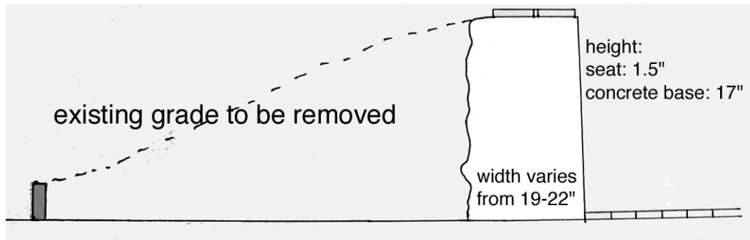
Section of existing bench and grade, drawing
