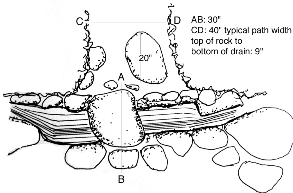
Plan Drawing
